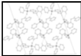
Fig. 2. Crystal packing of the title compound. Hydrogen bonds are drawn as dashed lines.
