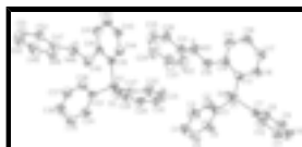
Fig. 1. The two independent molecules in the title compound with the atom-labeling scheme. Displacement ellipsoids are shown at the 40% probability level.
